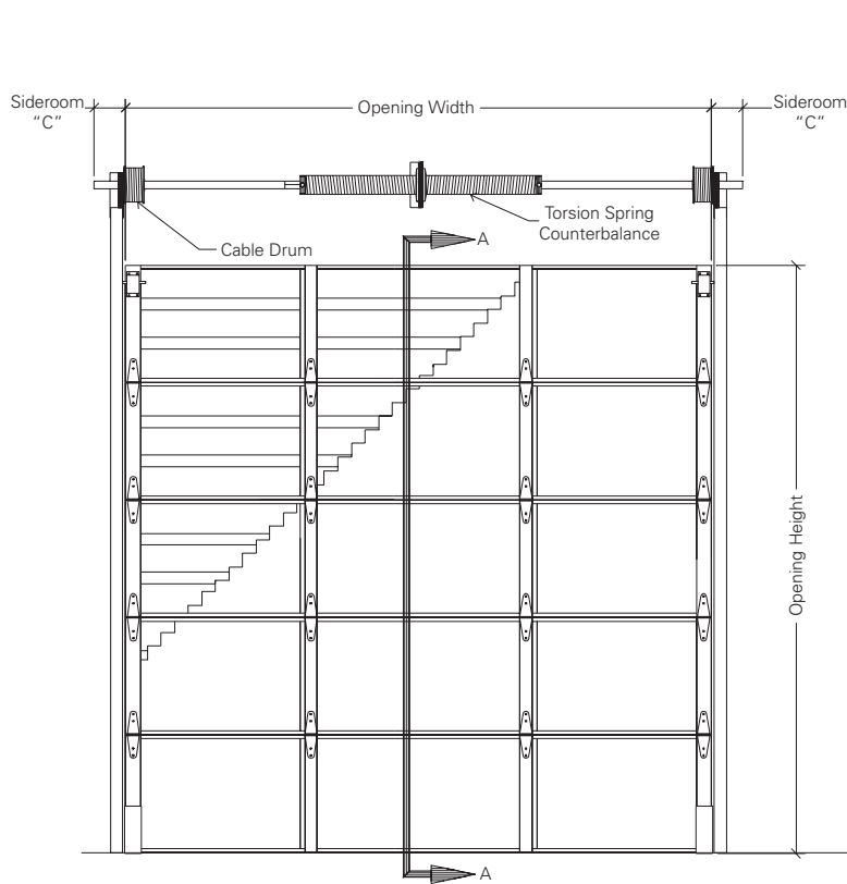
INTERIOR ELEVATION
